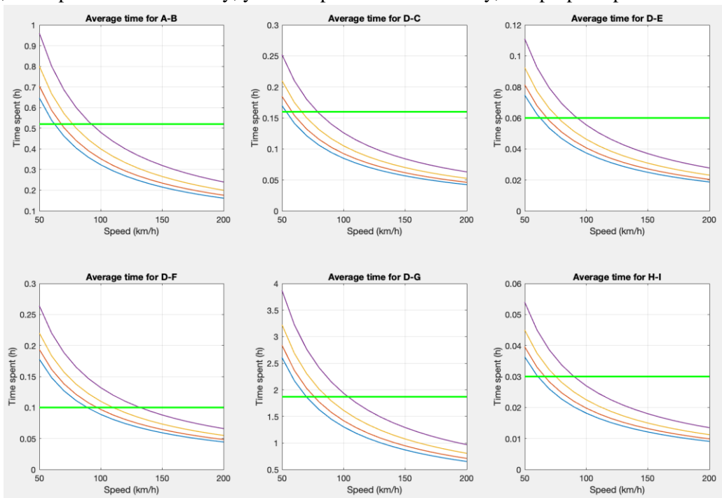
Fig. 5 Graph of time spent relative to the vehicle's average speed with considered delay
