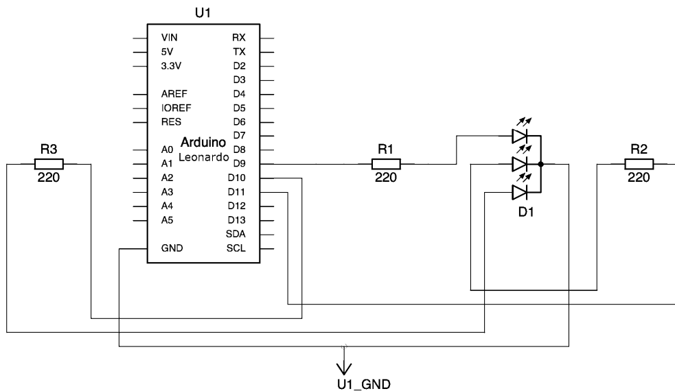
Fig. 2. Integrated Arduino Leonardo LED control circuit.
