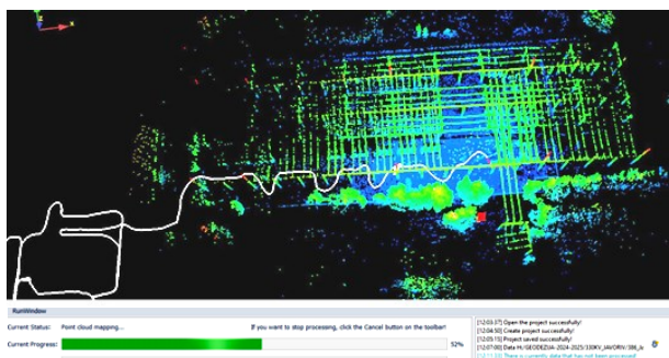
Fig. 12. Route visualization
