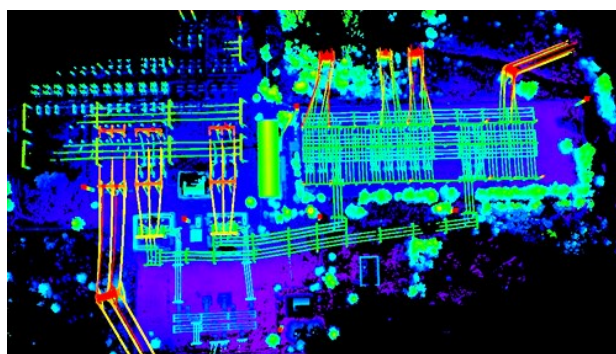
Fig. 13. Point cloud visualization following data processing in the SLAM GOpost software environment
