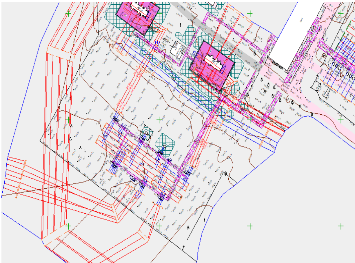
Fig. 20. Fragment of a topographic plan of the area at a scale of 1:500
