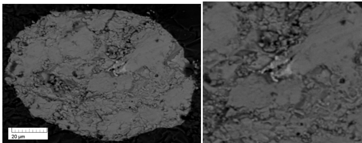
Fig. 12. Zircon with inclusions of baddeleyite (brighter) associated with Zr-poor silicate glass (darker), both on the right from the center. Crater No. 4 (#16132), BSE image (detail on the right).
