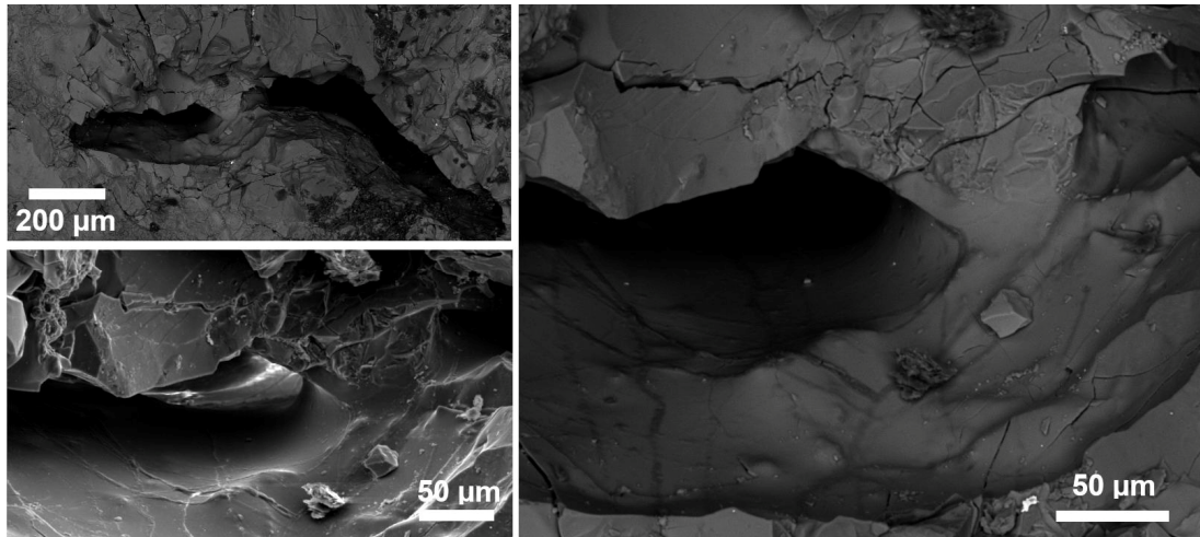
Fig. 3 A stretched bridge in a K-feldspar rich rock (Crater No. 4, granitic/syenitic? rock, #16133). Left top: overview in BSE (the irregular dark stainings are from a pencil), left bottom: detail in SE, right: detail in BSE (slightly darker quartz veinlets in the glass of K-feldspar composition).
