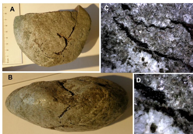
Fig. 1. A part of a fractured and deformed pebble with thin glass coating (sandstone, Crater No. 4, # 415).
