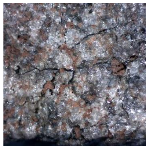
Fig. 7. Relatively thin fractures filled with glass (orthogneiss, Kaltenbach, #123; see also Fig. 4c) at the sheltered side which lacks any significant glass coating; surface depressions are filled with soil (image width 8 mm).
