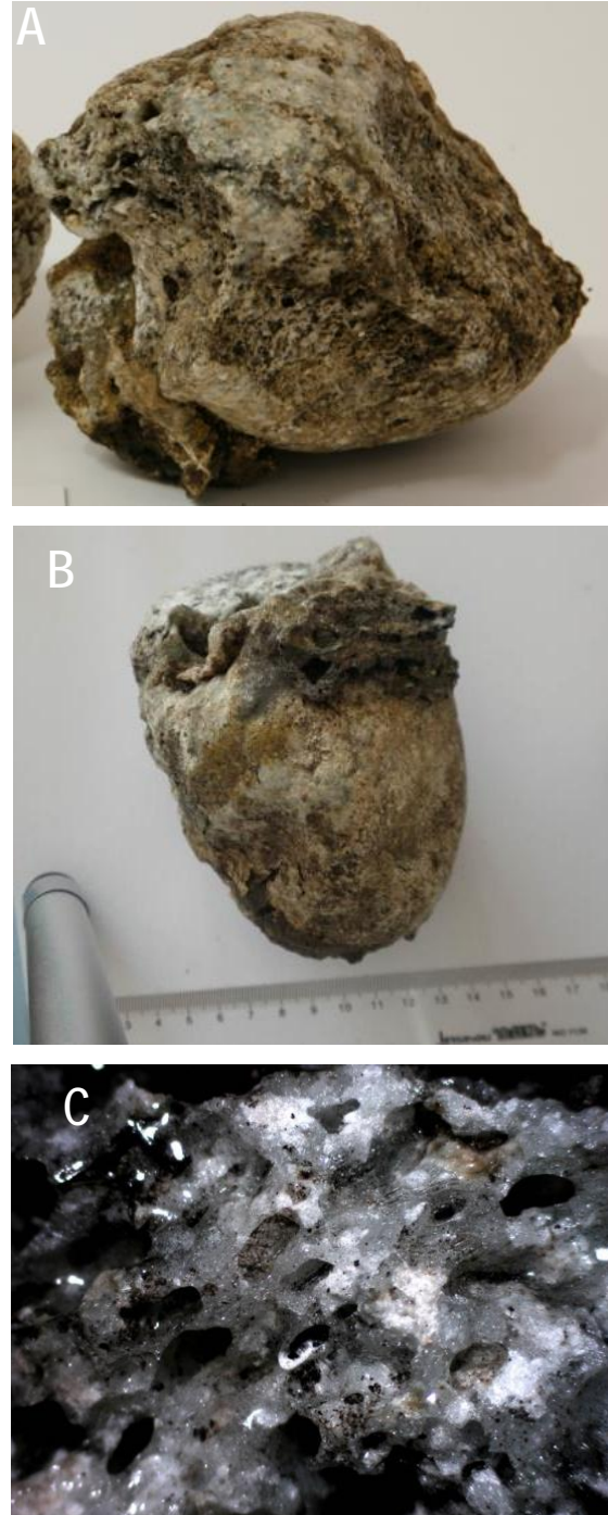
Fig. 10. Strongly expanded pebble (# 4/2-1). a), b) general view; see also the dark melt which is strongly deformed – possibly a secondary projectile: in a) in the left bottom, in b) in the top. c) original surface (relatively thin split on black background, 12x16 mm).
