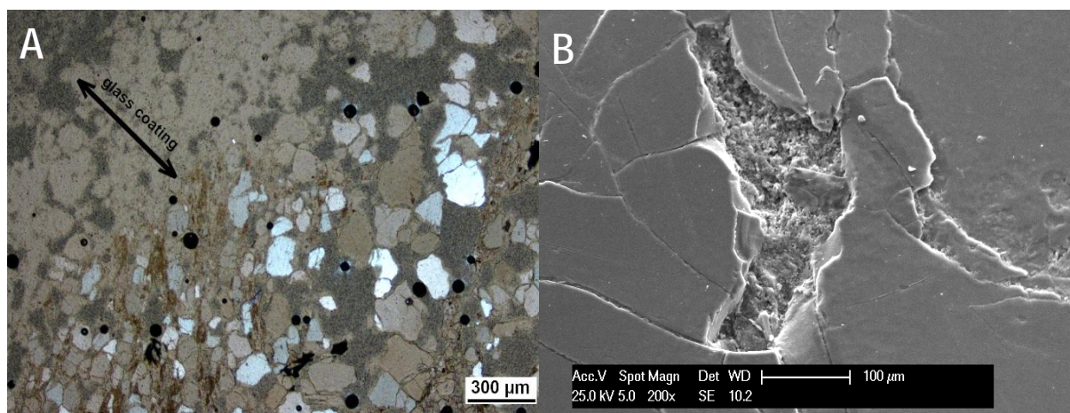
Fig. 18. A quartzite pebble (Crater No. 4, #15240) containing altered biotite and organic matter, with glass coating (independent on the foliation).
