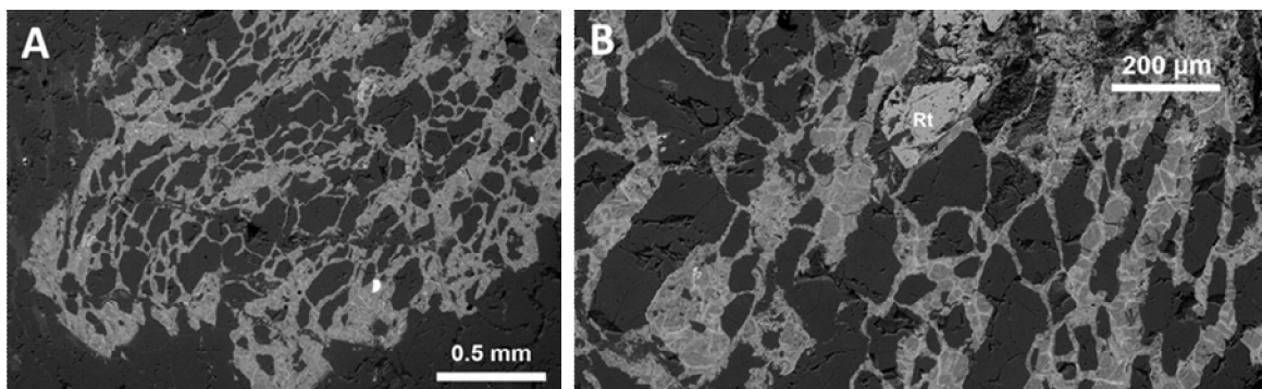
Fig. 14. Melt penetrations in quartzitic rock (Crater No. 5, #5/1/0a; BSE images).
