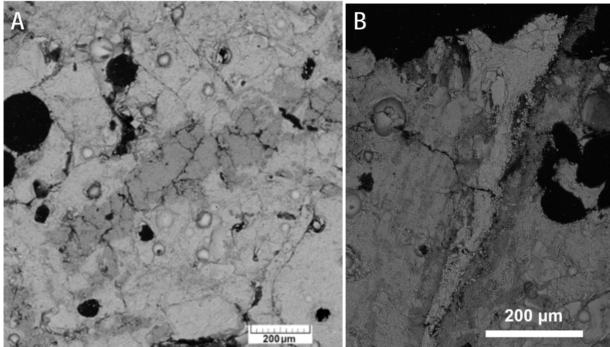
Fig. 13. Glasses of pure feldspar composition, Crater No. 4 (#16133, BSE images).
