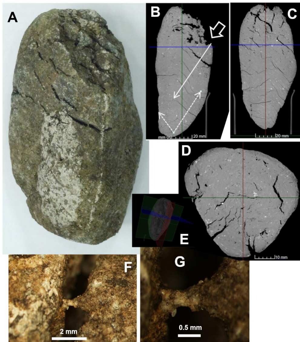
Fig. 2. A fractured pebble (Crater No. 4, #422) of quartzitic or granitic rock with stretched bridges in open fractures.
