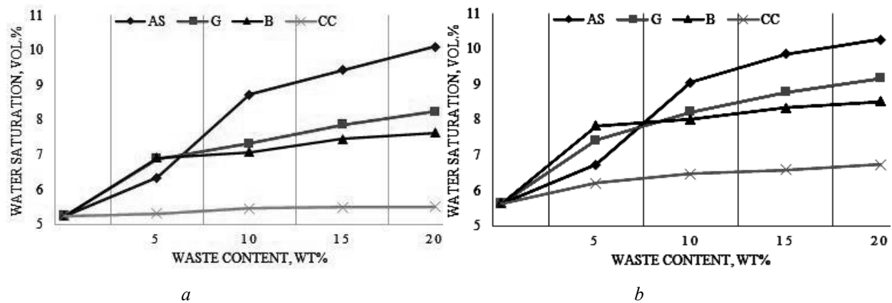
The influence of construction waste of different composition on the water saturation of road material samples after 7 days (a) and 28 days (b) of hardening
