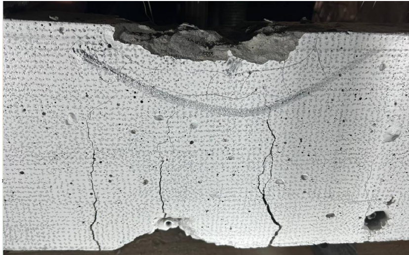
Figure 12. Concrete failure of the most compressed fiber.
