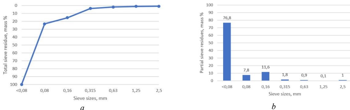
Fig. 3. Scattering curve (a) and fractional composition of wet fly ash (b)
