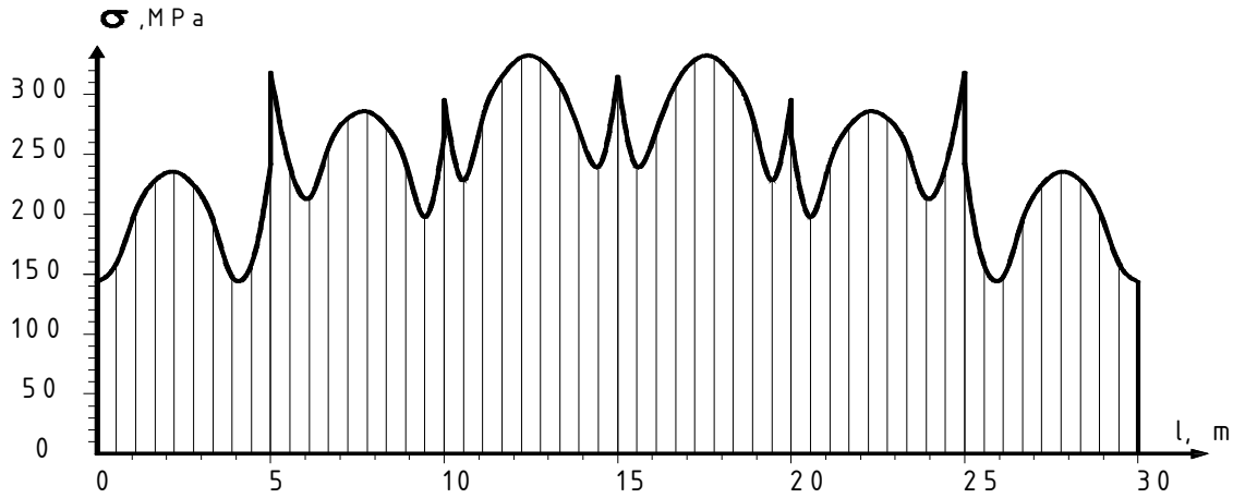
Fig. 5. Diagram of total normal stresses s in cross-sections of the stiffening girder of a combined truss with 6 panels with a span of 30 m
