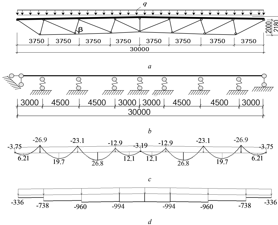
Fig. 6. Design diagram of a combined truss with a span of 30 m with eight stiffener beam panels (a); continuous eight-span stiffener beam with elastically compliant supports (b); diagram of moments in the stiffener beam – kN·m (c); diagram of longitudinal forces in the stiffener beam – kN (d)
