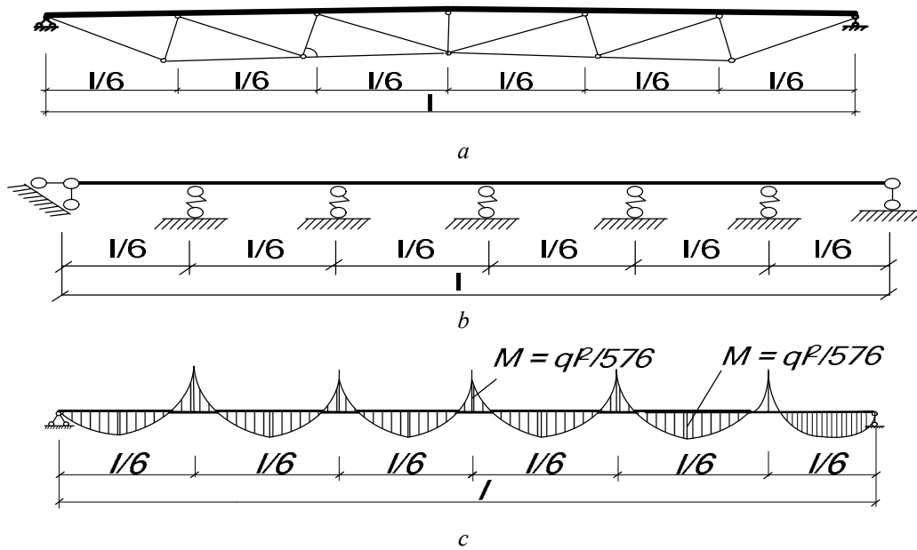
Fig. 3. Calculated scheme of a combined truss with a span of 30 m (a); continuous six-span stiffening girder with elastic-flexible supports (b); diagrams of bending moments in the stiffening girder – kNm (c)
