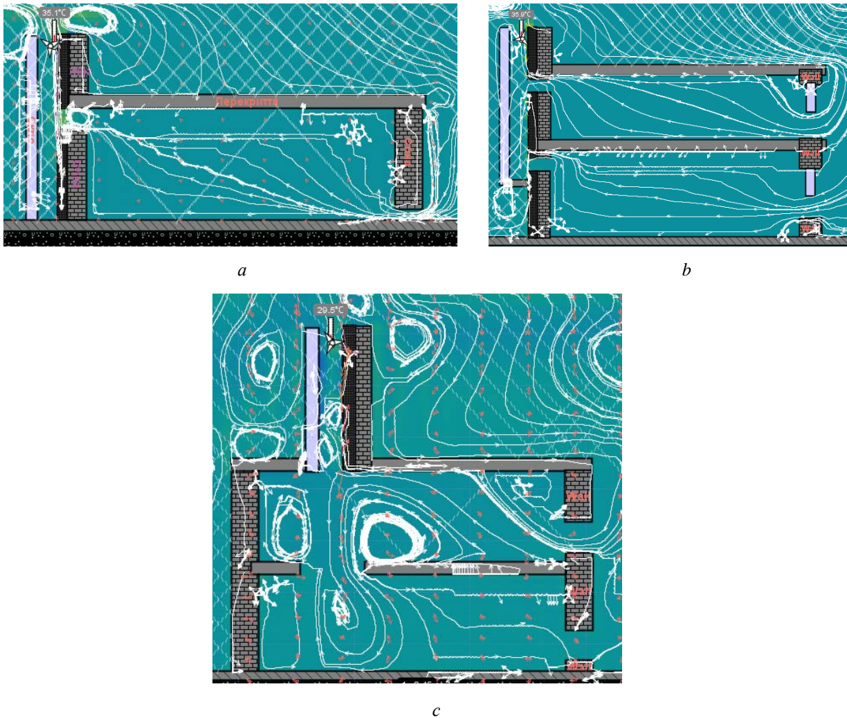
Fig. 1. Diagram of airflows around a building equipped with a Solar Chimney: a) a single-story building with an attached Solar Chimney and cross-ventilation; b) a two-story building with an attached Solar Chimney and cross-ventilation; c) a two-story building with a Solar Chimney integrated into the roof structure.
