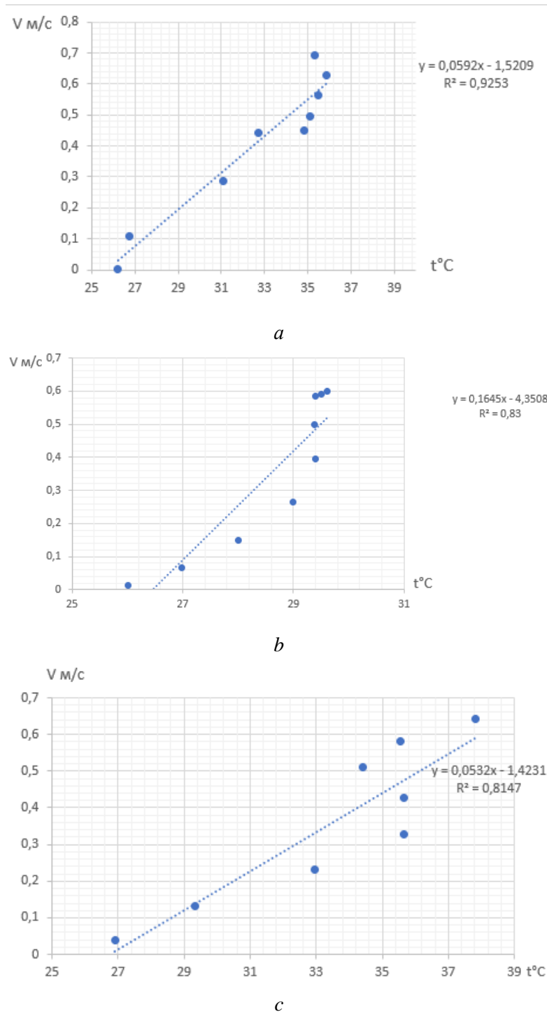
Fig. 2. Graph of air velocity change at the outlet of the solar chimney shaft versus exhaust air temperature
