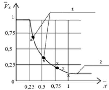
Fig. 2. Dependence of relative axial velocity on relative longitudinal coordinate
