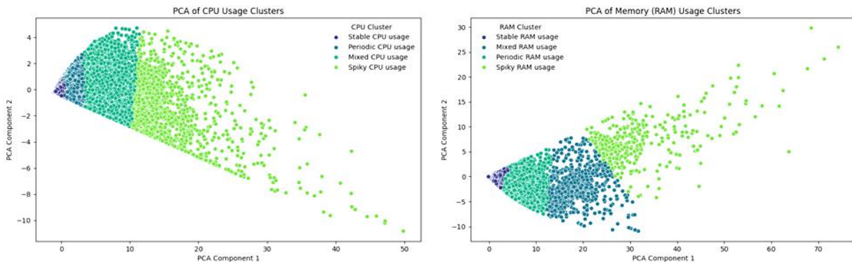
Fig. 1. PCA visualization of CPU and memory utilization clusters
