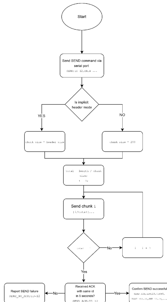
Fig. 6. Block diagram of the segmented guaranteed data transfer algorithm
