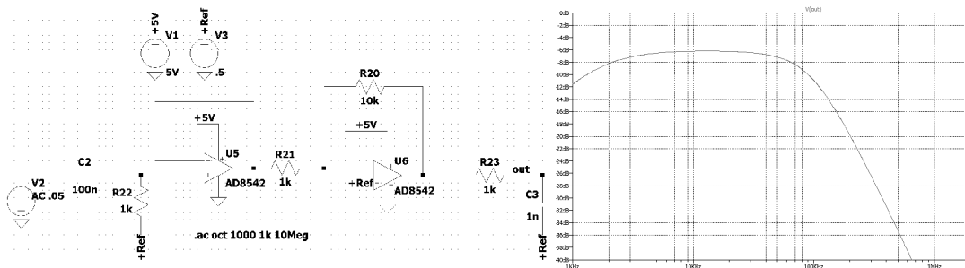
Fig. 22. BPF simulation setup
