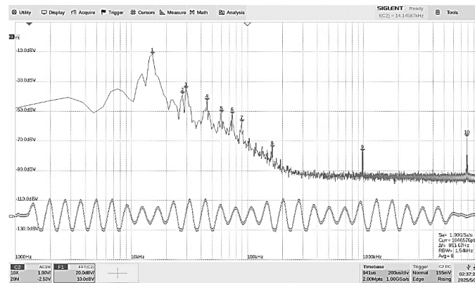
Fig. 25. PLC host to PLC node signal waveform and FFT. THD+N = 8.6 %, SNR = 52.5 dB
