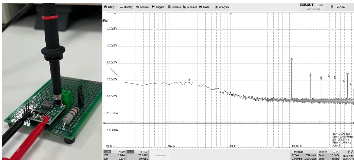
Fig. 18. Unmodulated DC-DC signal waveform and FFT
