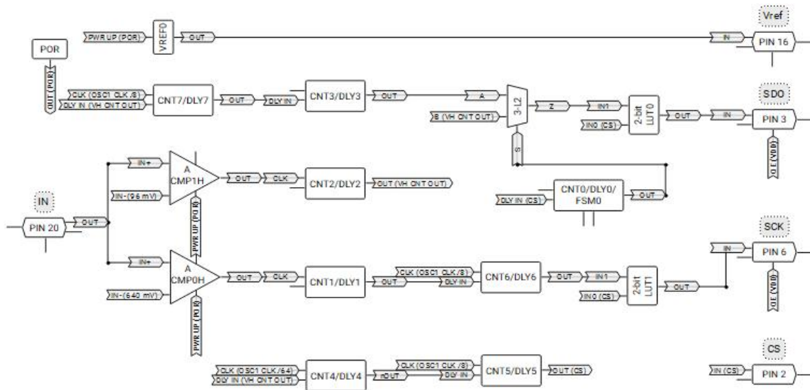
Fig. 26. ASK to SPI decoder design
