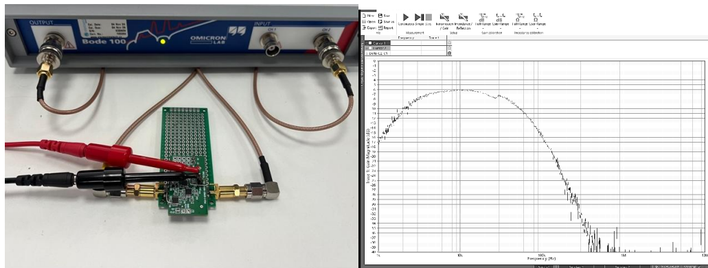
Fig. 23. BPF block measurement setup
