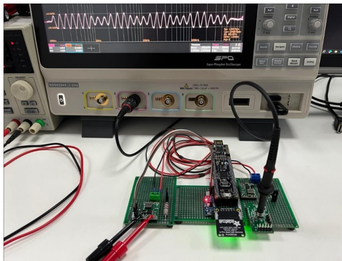
Fig. 24. PLC host to PLC node signal quality measurement setup
