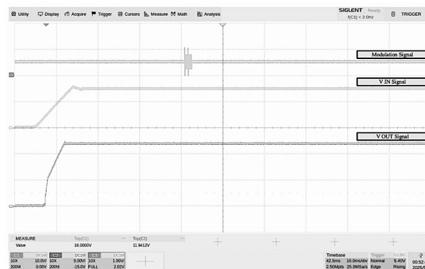
Fig. 16. PLC host operating waveform
