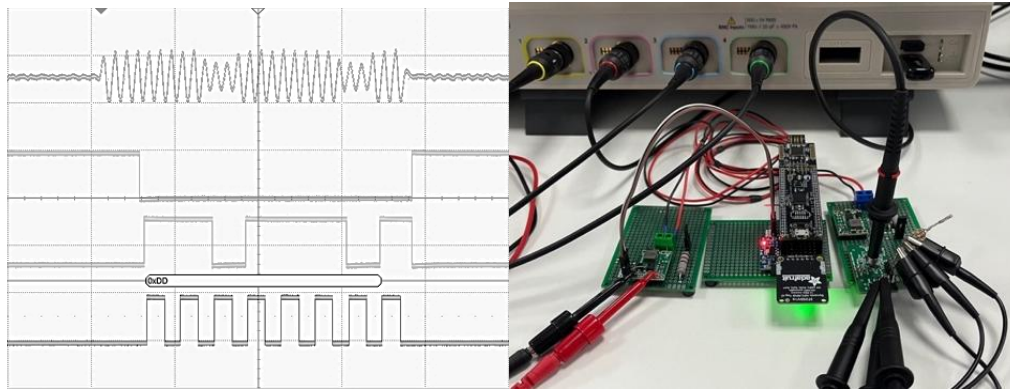
Fig. 27. (Continuation). ASK to SPI decoder bench testing results
