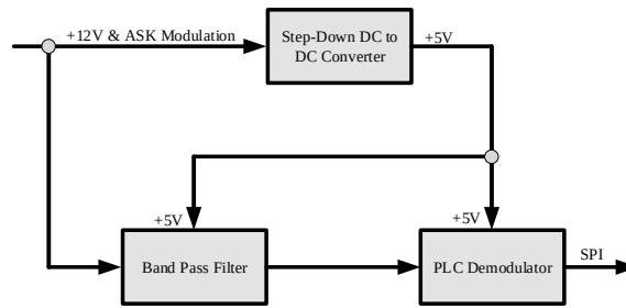
Fig. 20. PLC node block diagram
