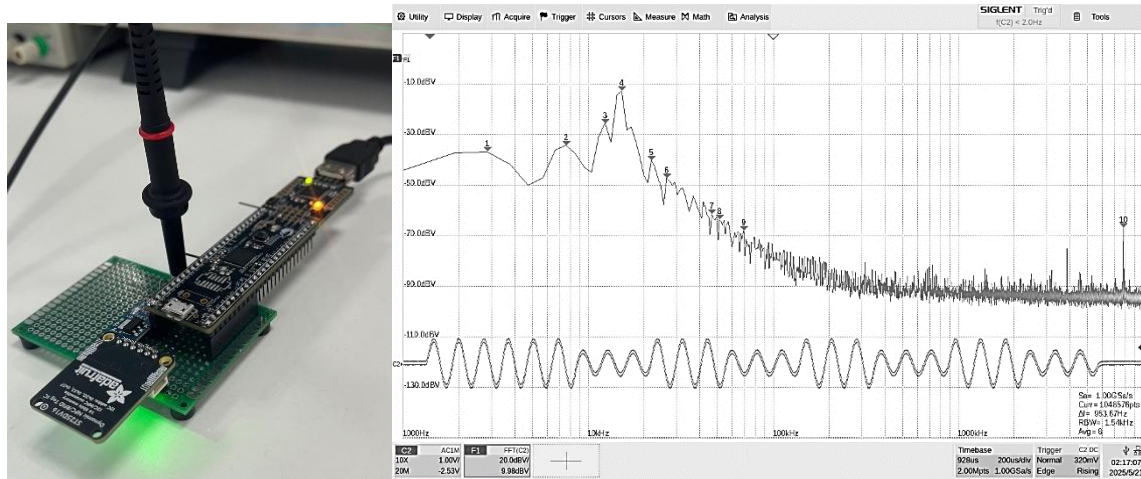
Fig. 17. PLC injection signal waveform and FFT, THD+N =4.8
