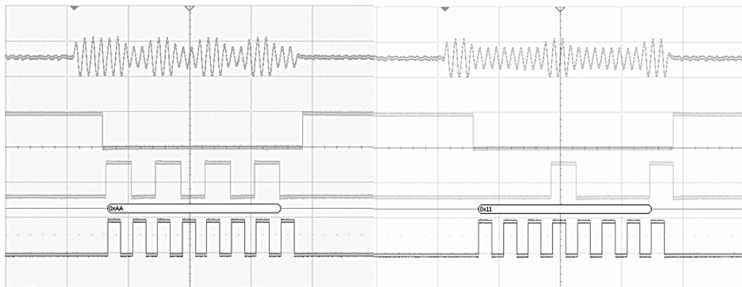
Fig. 27. ASK to SPI decoder bench testing results
