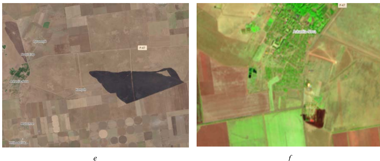
Fig. 3. (Continuation). Pyrogenic events in the Askania-Nova Reserve during: a – 30.07.2022; b – 29.08.2022; c – 27.03.2023; d – 24.08.2023; e – 08.09.2023; f – 28.09.2023
